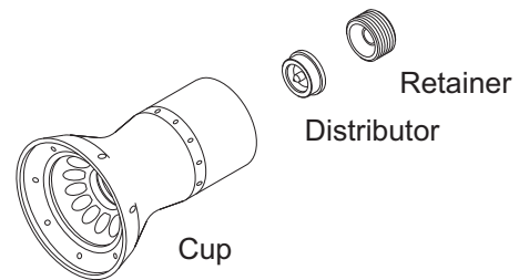
Distributor
