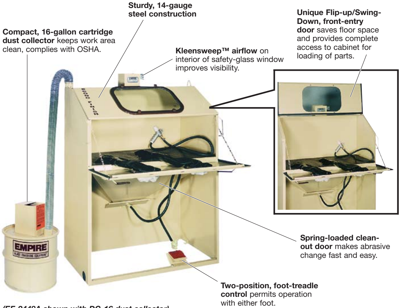
(EF-2448A shown with DC-16 dust collector)
